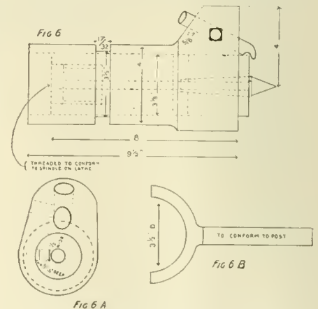
TURNING TOOL FOR LIFTING SHAFT JOURNALS.
